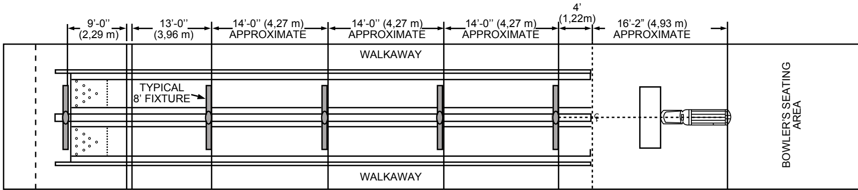
TYPICAL FOUR TIER LIGHTING PLAN
